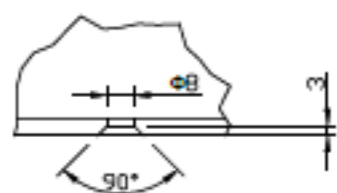
A (1:2)
